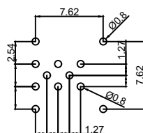
Pcb plate opening size (PCB板开孔尺寸)
