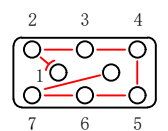
M-directional layout (M向排版位)
