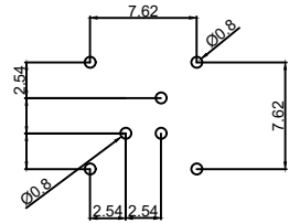
Pcb plate opening size (PCB板开孔尺寸)
