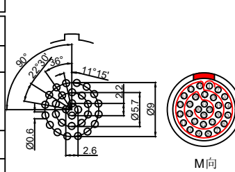
Pcb plate opening size (PCB板开孔尺寸)
