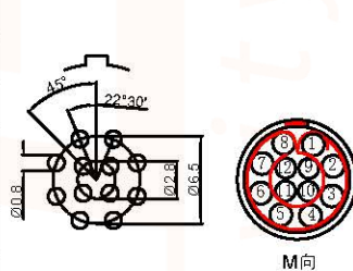
Pcb plate opening size (PCB板开孔尺寸)
