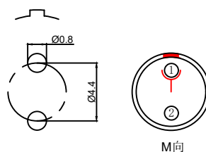
Pcb plate opening size (PCB板开孔尺寸)
