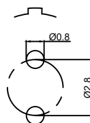
Pcb plate opening size (PCB板开孔尺寸)
