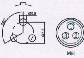
Pcb plate opening size (PCB板开孔尺寸) Pane hole size (面板开孔尺寸)
