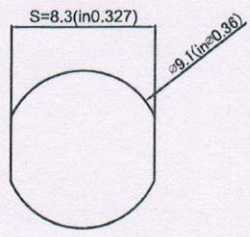
Pcb plate opening size (PCB板开孔尺寸) Pane hole size (面板开孔尺寸)
