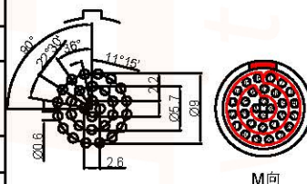
Pcb plate opening size (PCB板开孔尺寸)
