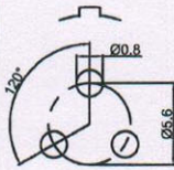
Pcb plate opening size (PCB板开孔尺寸)
