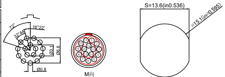
Pcb plate opening size (PCB板开孔尺寸)
