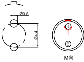
Pcb plate opening size (PCB板开孔尺寸)
