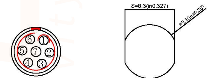
Welded surface (焊接面)
