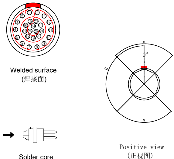
Welded surface (焊接面)
