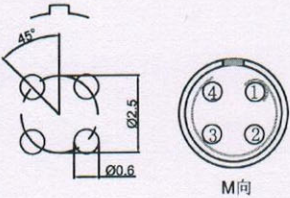
Pcb plate opening size (PCB板开孔尺寸)
