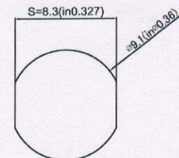
Pane hole size (面板开孔尺寸)
